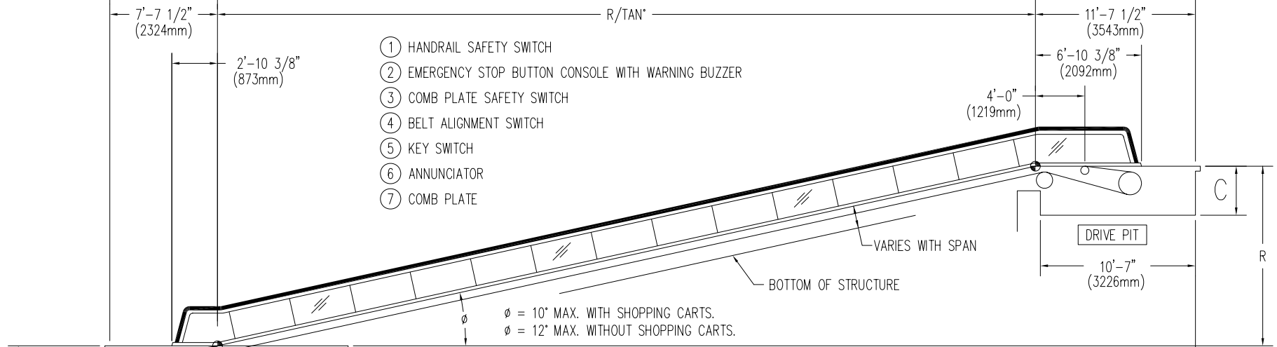
SPEEDRAMP ELEVATION
